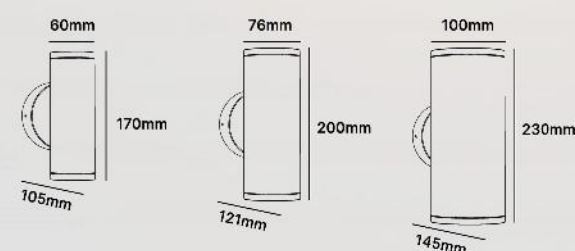
W43-10W
